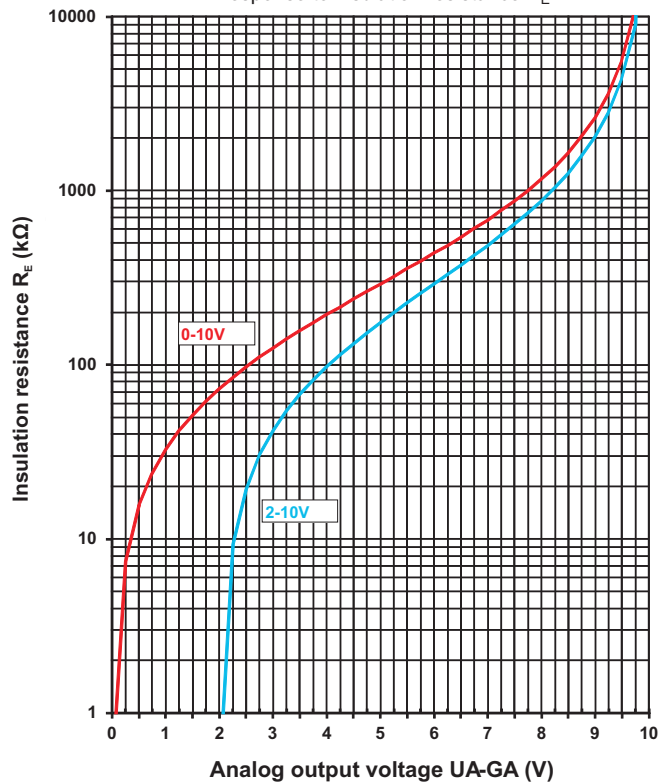
Analog output voltage UA-GA in response to insulation resistance R_E
