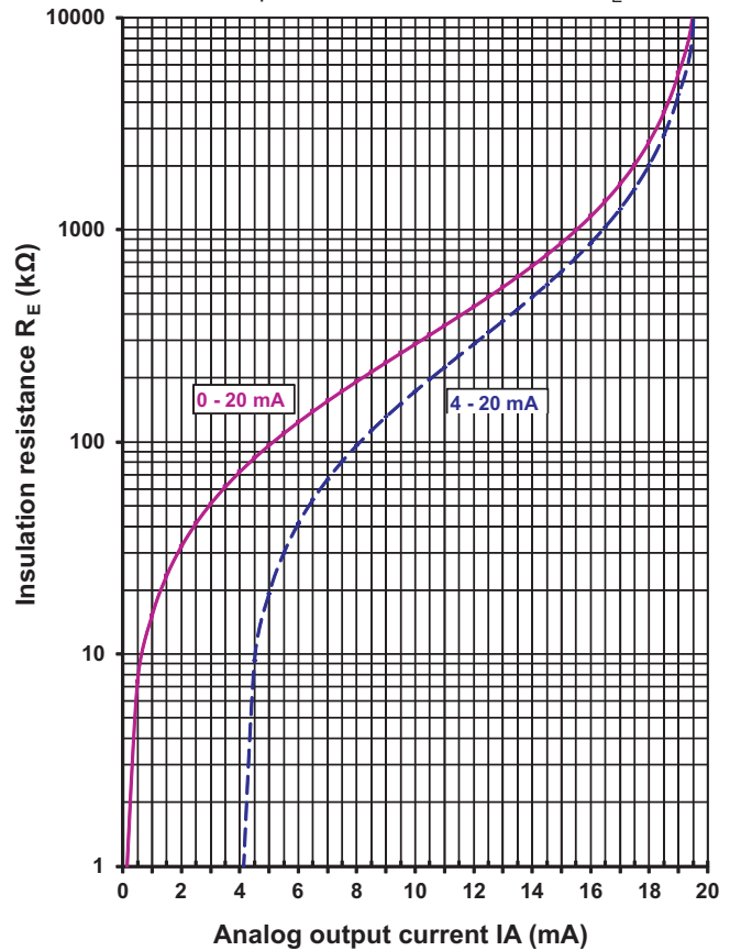
Analog output current IA in response to insulation resistance R_E
