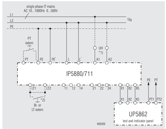
Monitoring of a single phase IT power system with test and indicator panel
