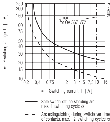
OA 5672, OA 5682: Limit curve for arc-free operation (at t u = 20°C)
