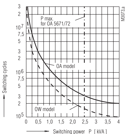
OA 5672, OA 5682: Contact service life (at t u = 20°C)
