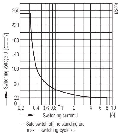
OA 5668: Limit curve for arc-free operation (at t u = 20°C)
