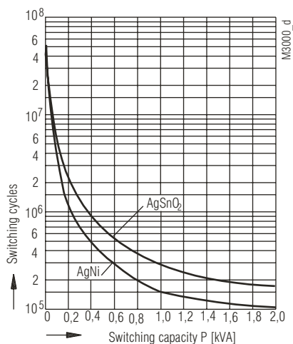
OA 5668: Contact service life (at t u = 20°C)
